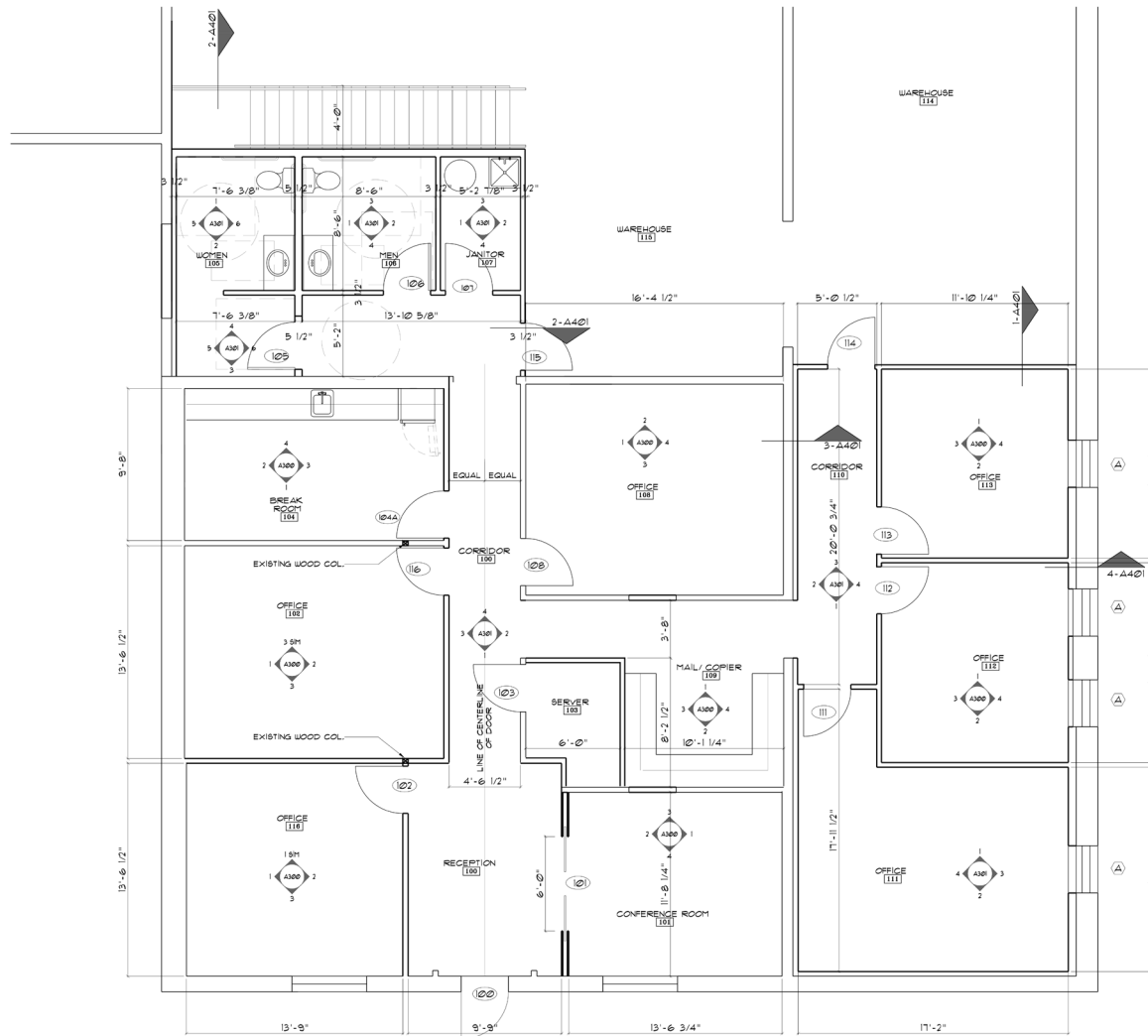
FLOOR PLAN 1/4"=1'-0" 01 A101
