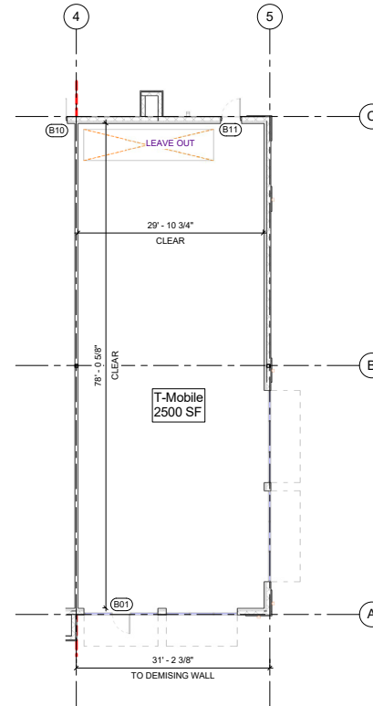
② Lease Plan - T-Mobile 1/8" = 1'-0"
